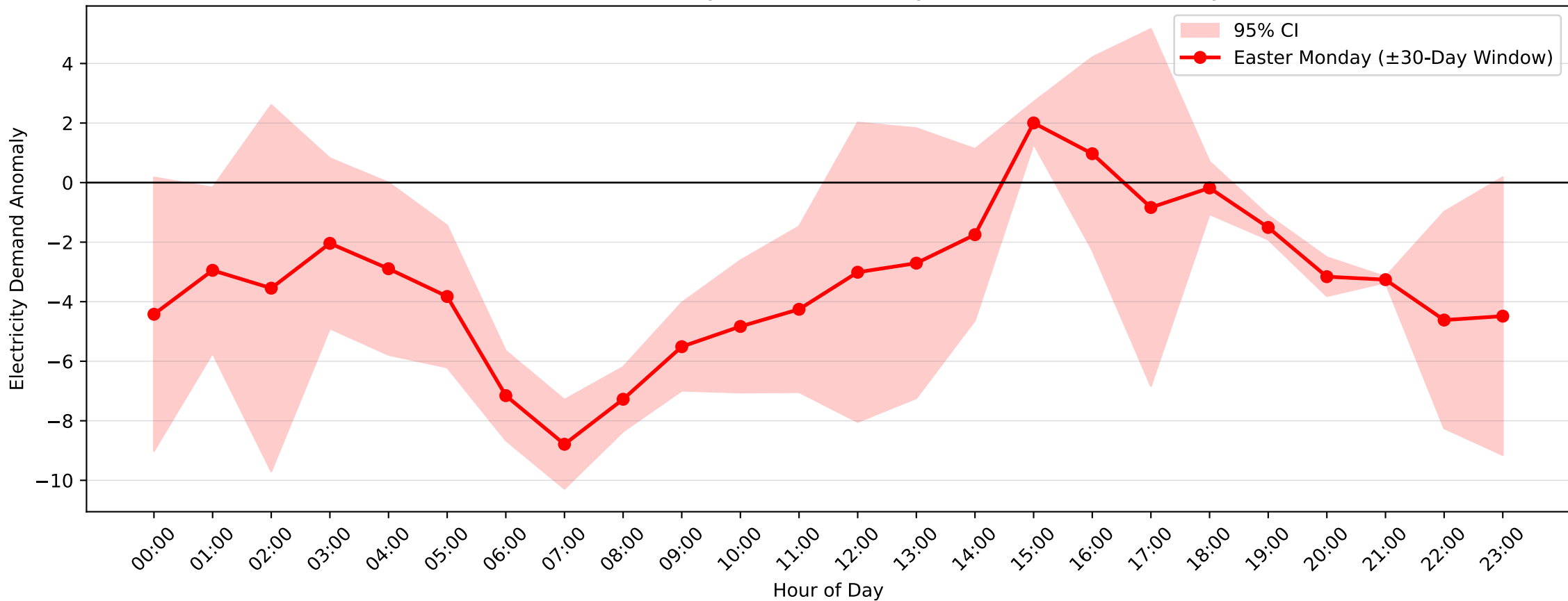
Meadowbank Demand Anomaly: Easter Monday (2011-2012, \pm 30 -Day Window)
