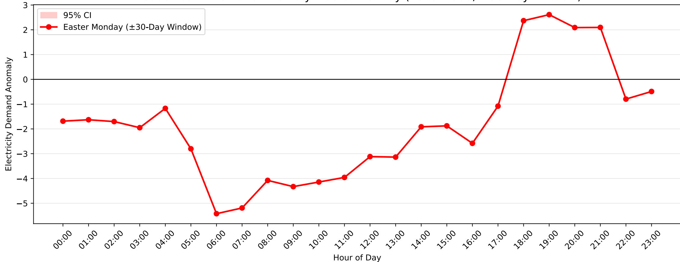
Meadowbank Demand Anomaly: Easter Monday (2005-2006, \pm 30 -Day Window)
