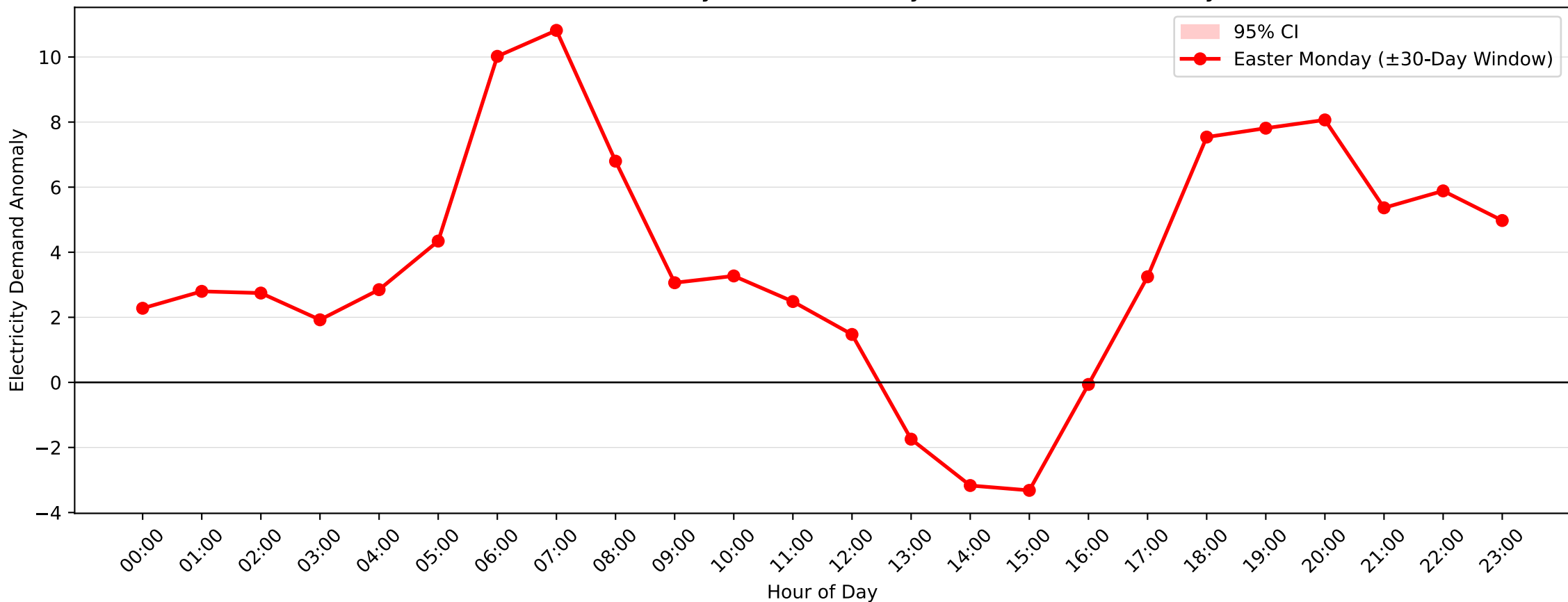
Meadowbank Demand Anomaly: Easter Monday (2004-2005, \pm 30 -Day Window)
